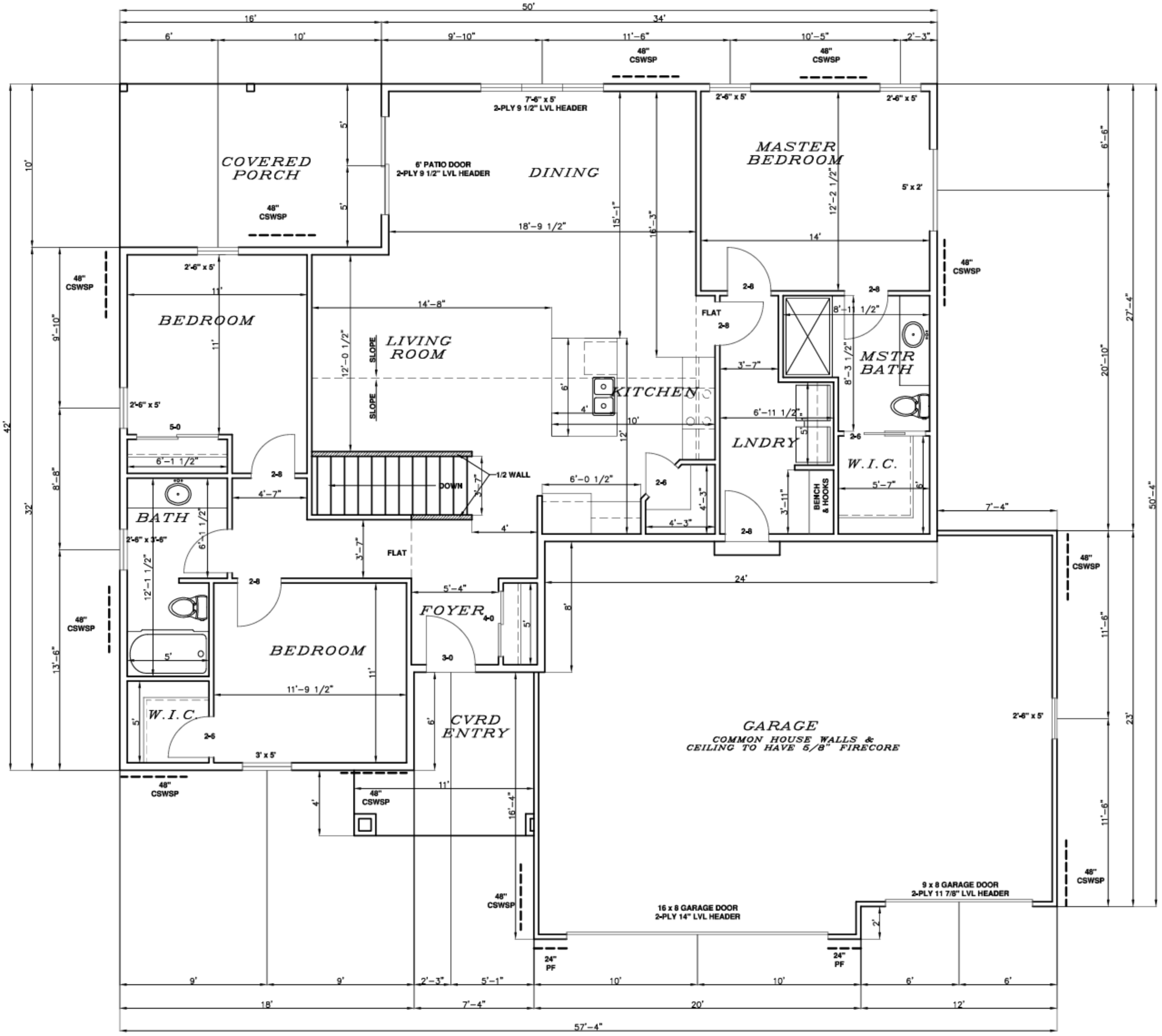
FLOOR PLAN 1/4" = 1' 1556 SQ. FT.
