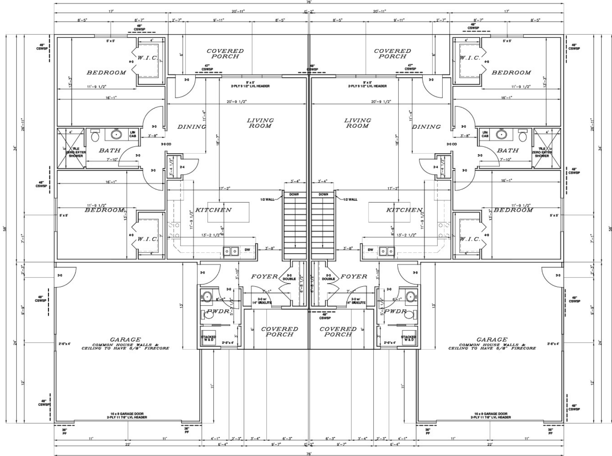
FLOOR PLAN \frac{1}{4}" = 1' 1322 SQ.FT. / SIDE
