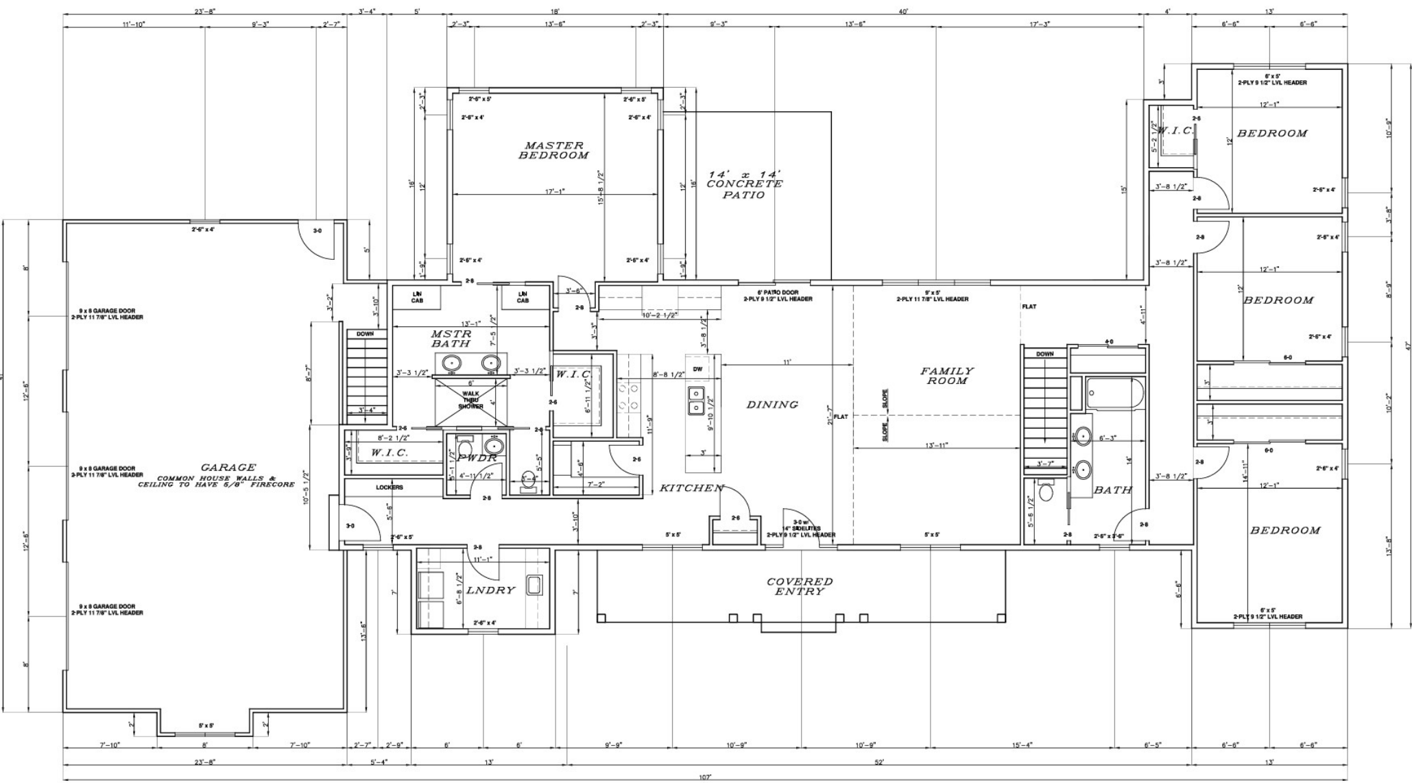
FLOOR PLAN 1/4" = 1' 2592 SQ.FT.
